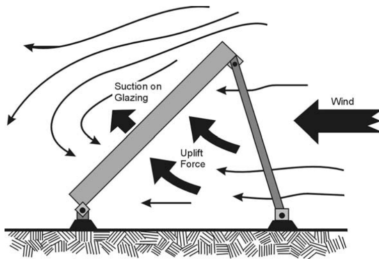
Figure 2 Conceptual drawing of wind loading
