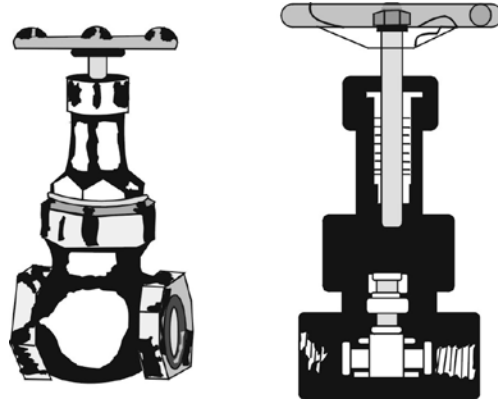
Figure 31 Gate valve
