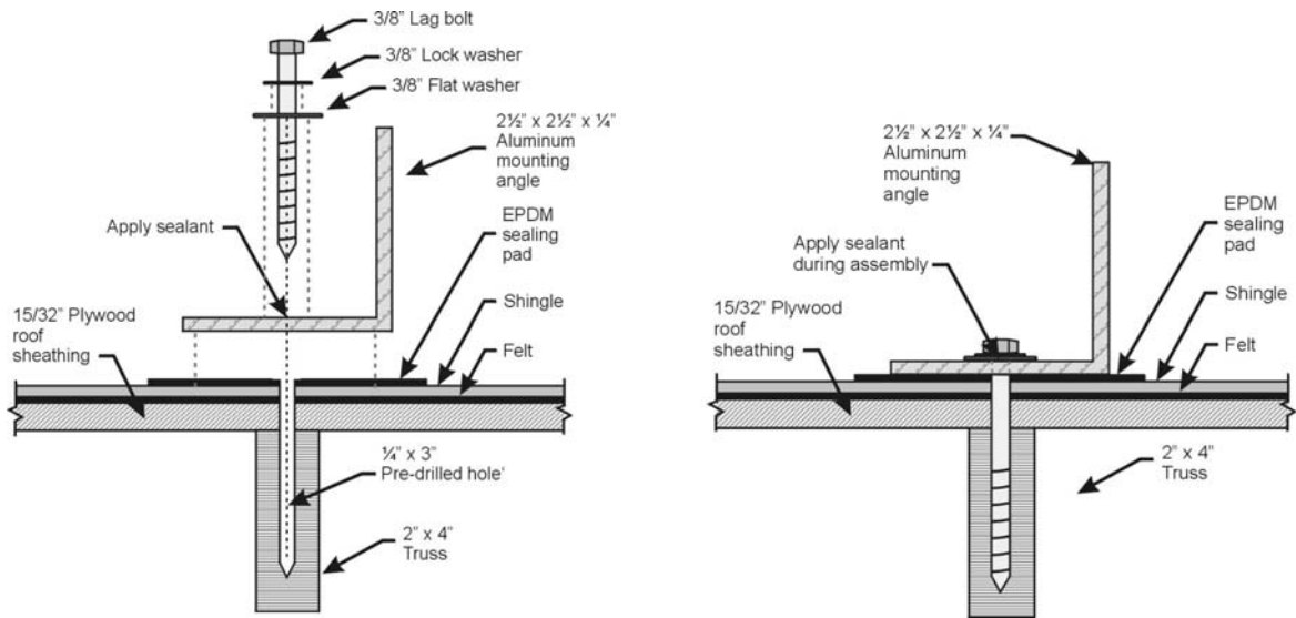
Figure 16 Lag-bolted mounting assembly
