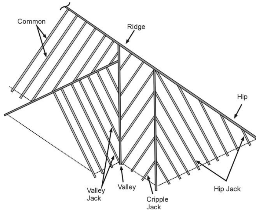
Figure 9 Roof structures
