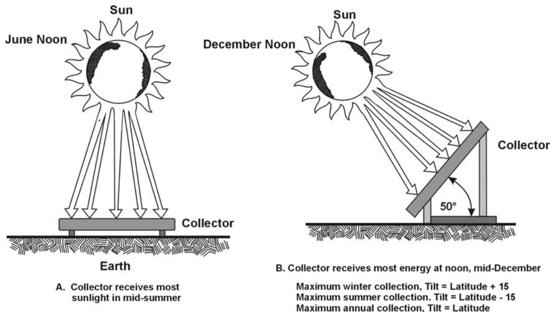
Figure 6a And 6b. Collected Energy Varies with Time of Year And Tilt
