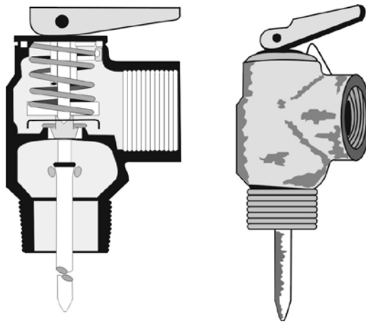
Figure 26 Pressure-temperature relief valve
