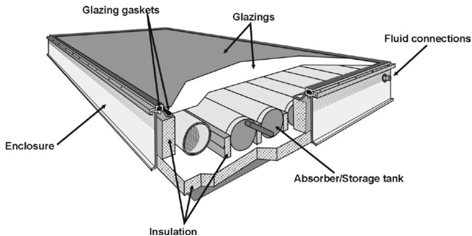
Figure 4 ICS collector
