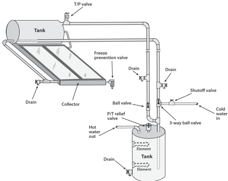
Figure 7 Direct thermosiphon system
