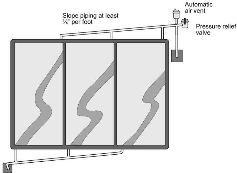
Figure 24 Piped and vented collector array
