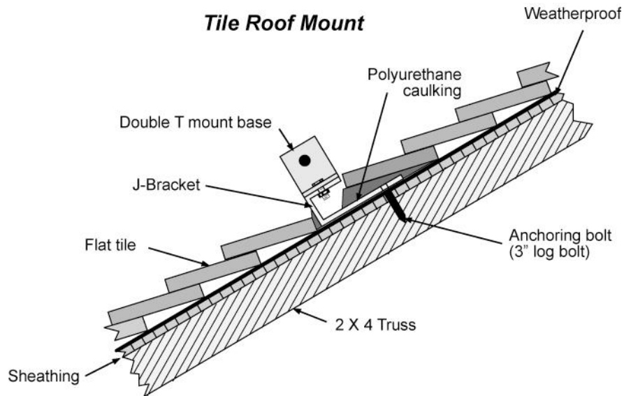
Figure 12 Tile roof-bracket mounting
