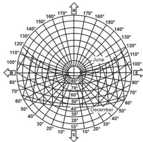
Sun Paths in the sky at 28^\circ latitude.
