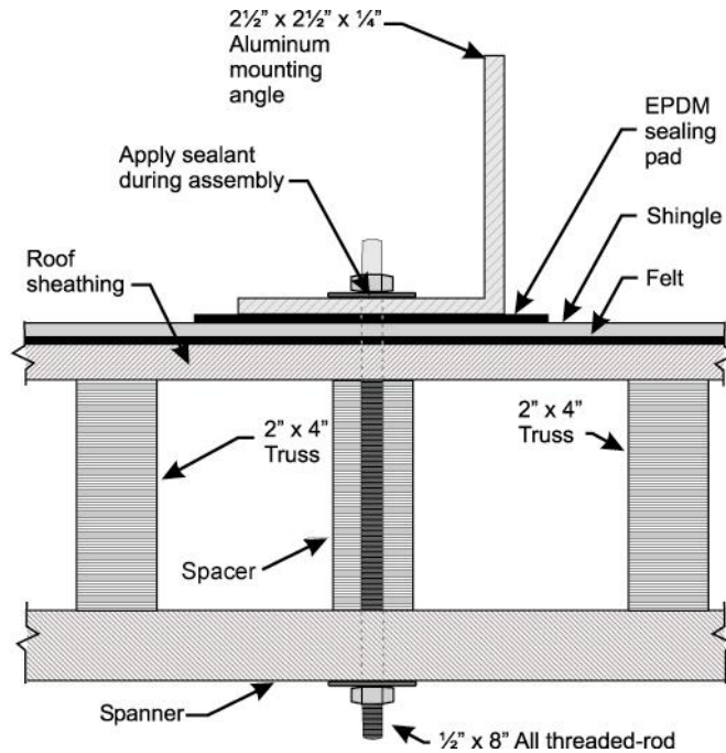
Figure 15 Spanner mounting
