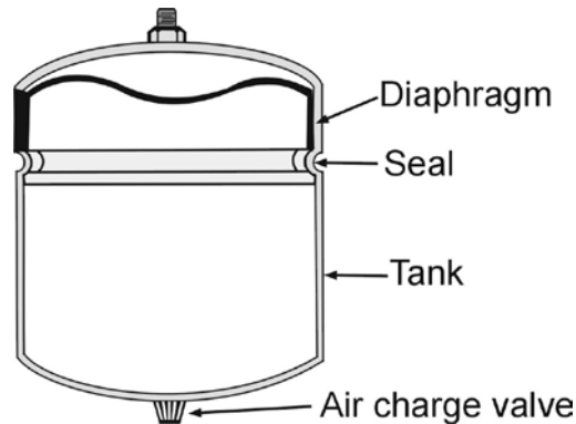
Figure 23 Expansion tank
