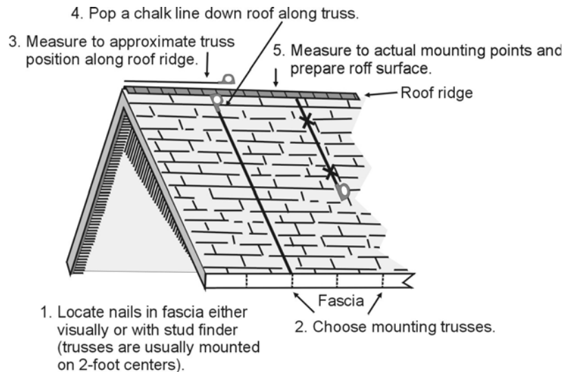
Figure 10 A method of locating mounting points
