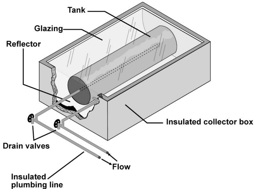
Figure 5 Batch collector
