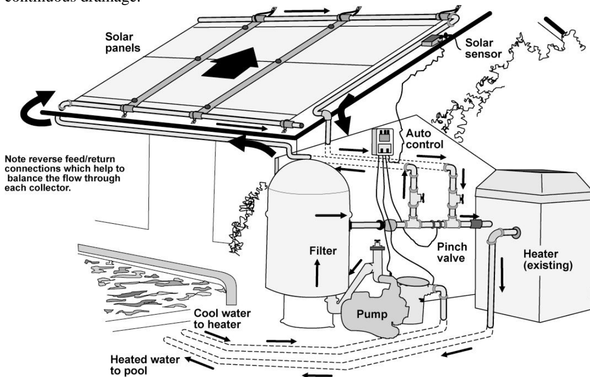
Figure 9 Plumbing schematic
