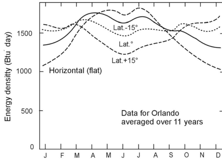
Figure 8. Various Collector Tilt Angles
