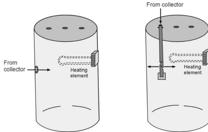
Figure 4 Side port and “dip tube” arrangement of collector return port
