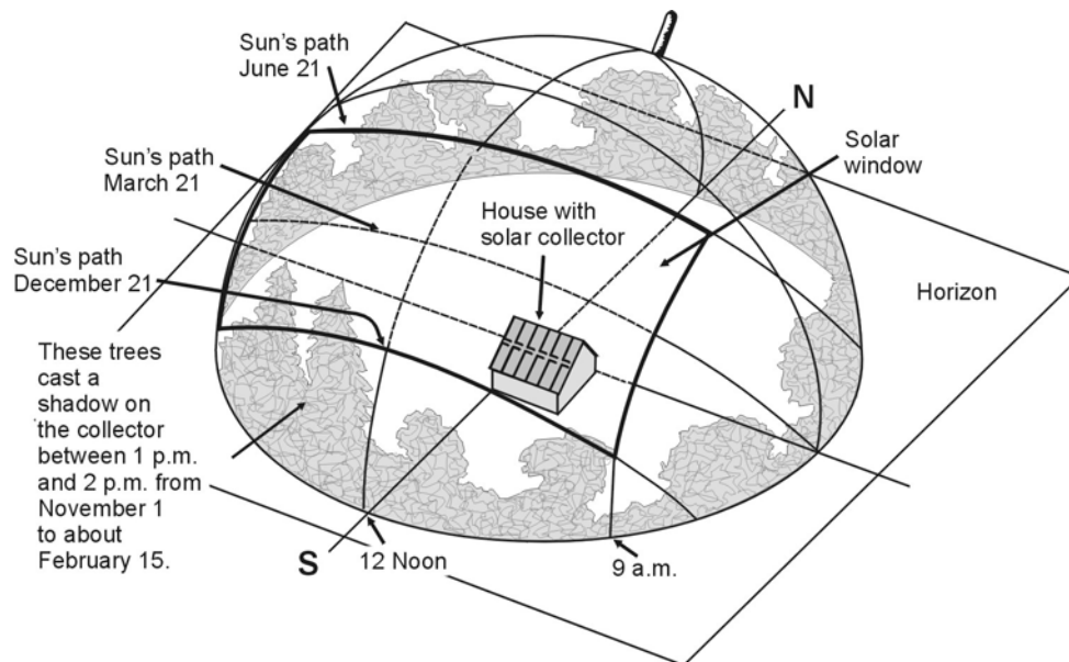
Figure 1 Solar window
