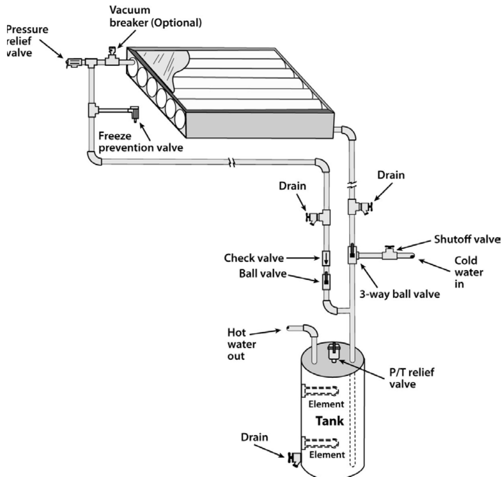
Figure 9 Integral collector storage (ICS) system
