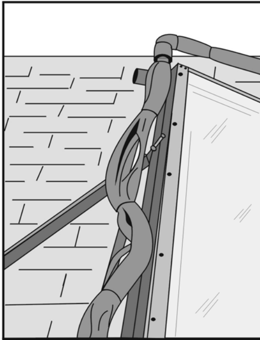
Figure 12 Plastic insulation should not be used in high temperature or external applications
