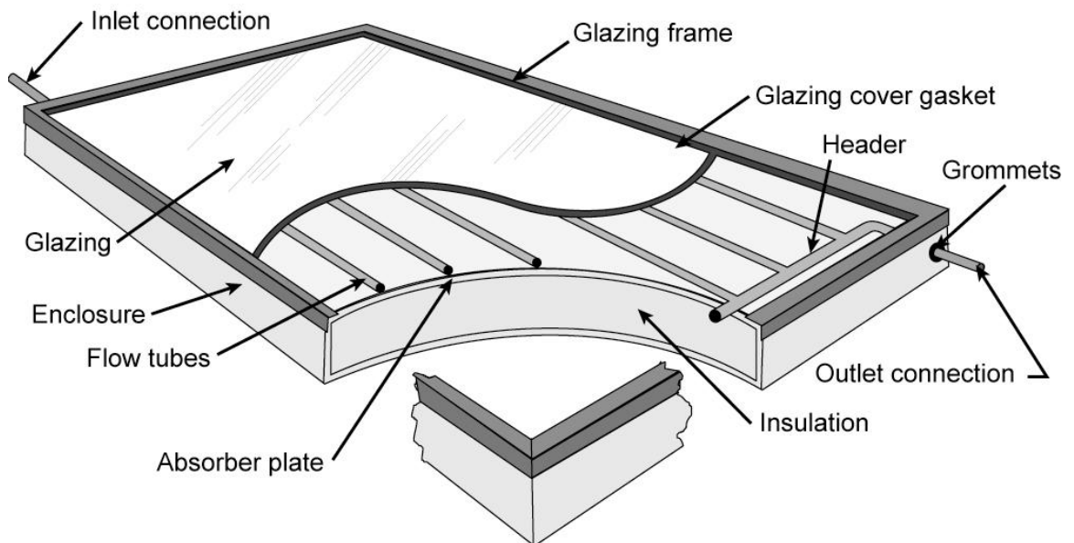
Figure 1 Flat plate collector
