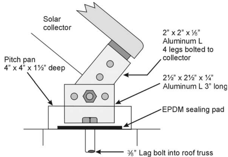
Figure 14 Pitch pan detail
