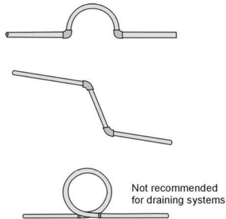
Figure 1 Expansion loops – systems must be able to drain
