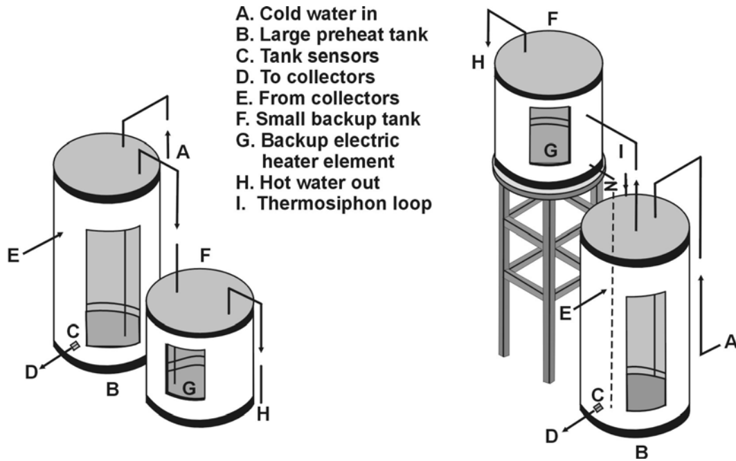
Figure 2 Multiple tank connection
