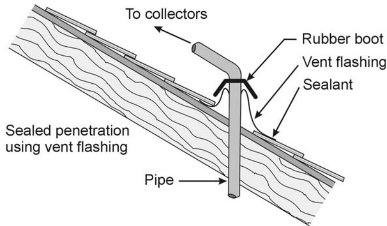
Figure 18 Penetration with vent stack flashing
