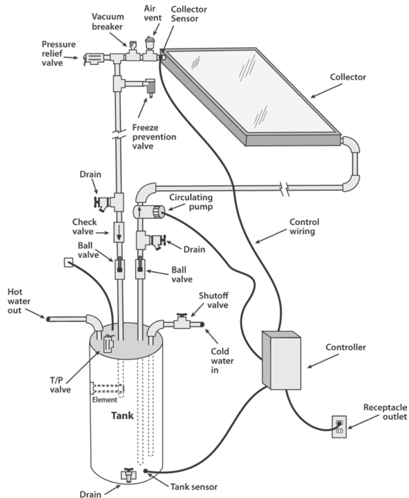
Figure 3 Active direct system with differential controller
