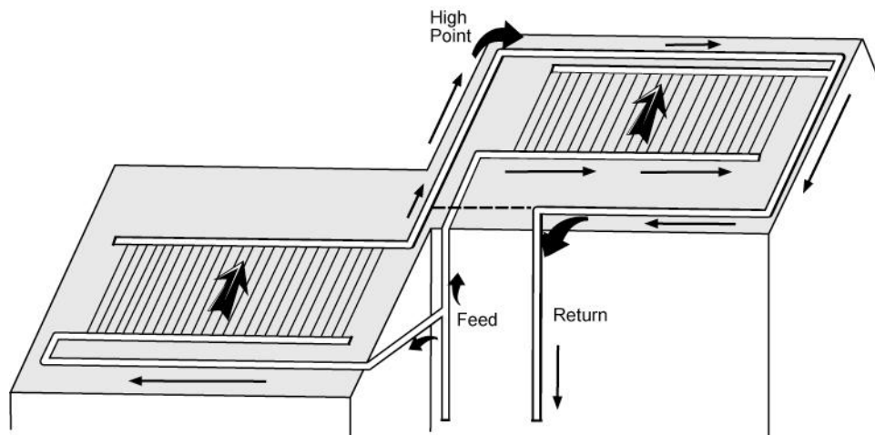
Figure 22 Plumbing collectors at different heights
