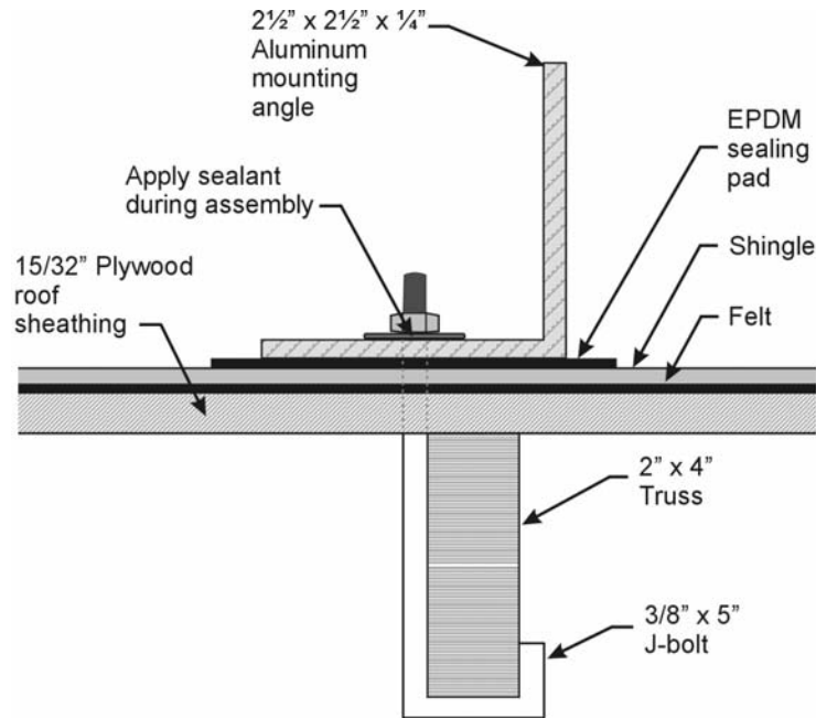
Figure 17 J-bolt mounting
