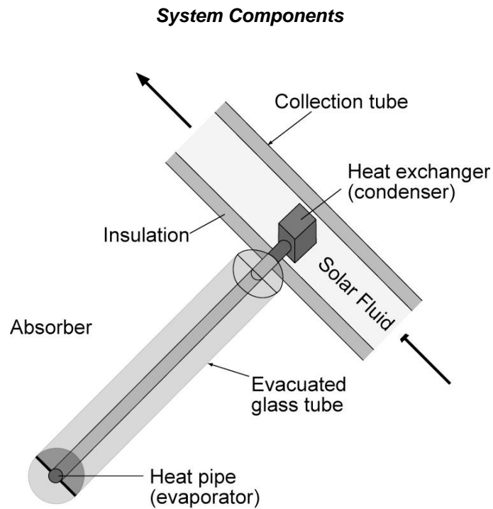
Figure 3 Heat pipe evacuated-tube collector
