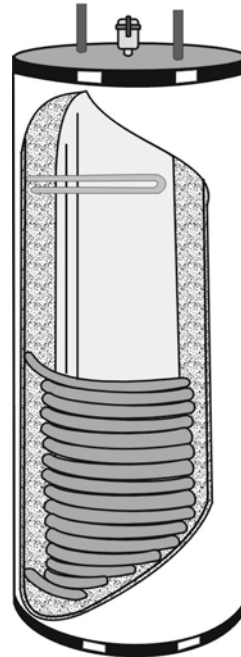
Figure 20 Wraparound type heat exchanger
