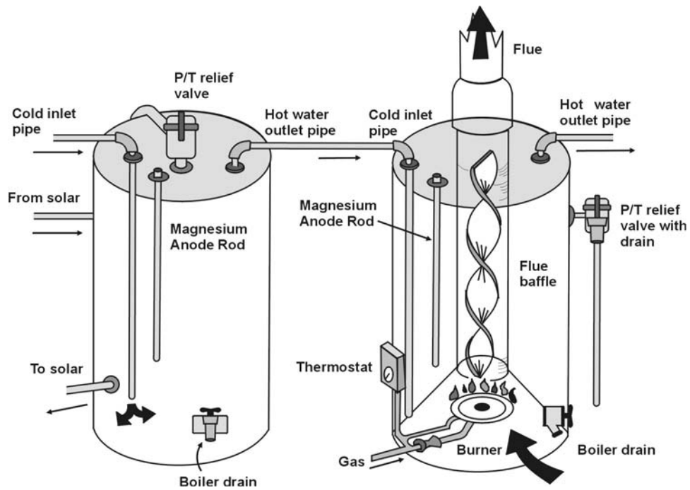
Figure 3 Gas heater connection
