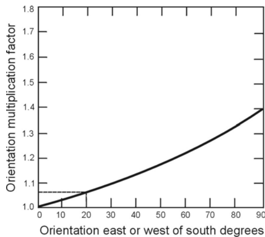
Figure 7. Glazed Collector Orientations
