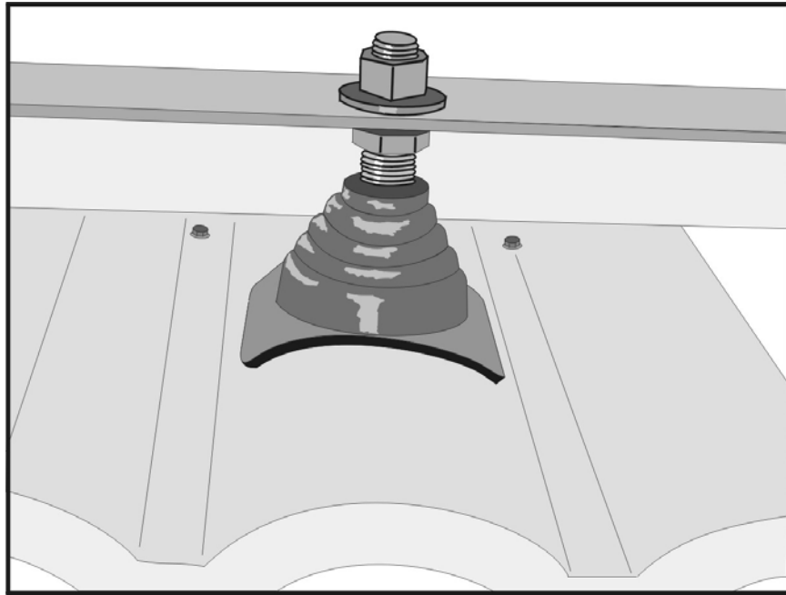
Figure 11 Tile roof mount
