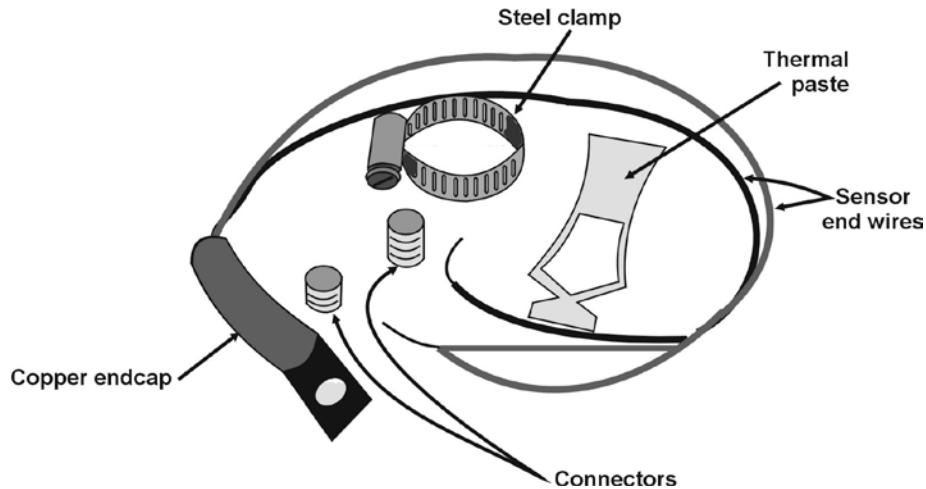
Figure 14 Sensors
