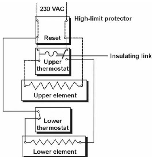
Typical electrical connections in a tank with two heating elements
