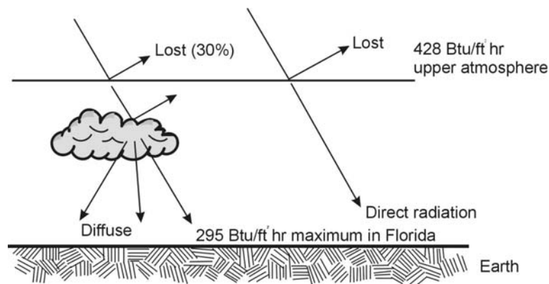
Figure 2. Atmospheric Effects on Solar Energy Reaching Earth
