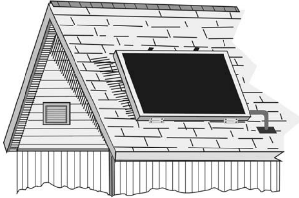
Figure 3 Collector mounted down from roof ridge to reduce wind loading and heat losses
