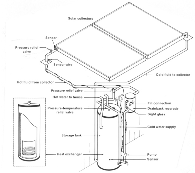
Figure 13 Drain-back system with internal tank heat exchanger
