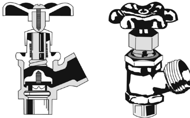
Figure 32 Drain valve
