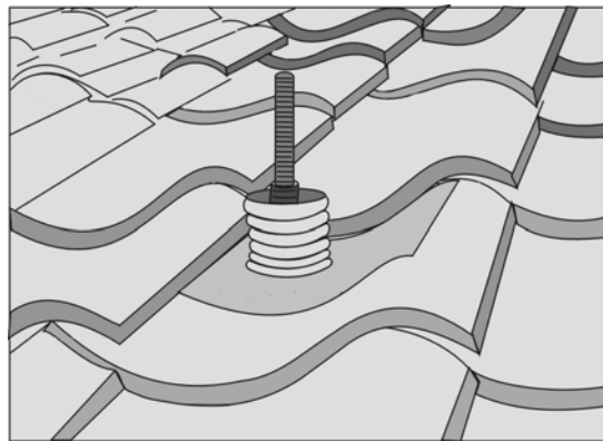
Figure 13 Vent stack flashing
