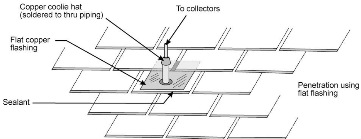
Figure 19 Penetration with flat flashing
