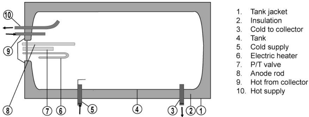
Figure 7 Horizontal solar storage tank
