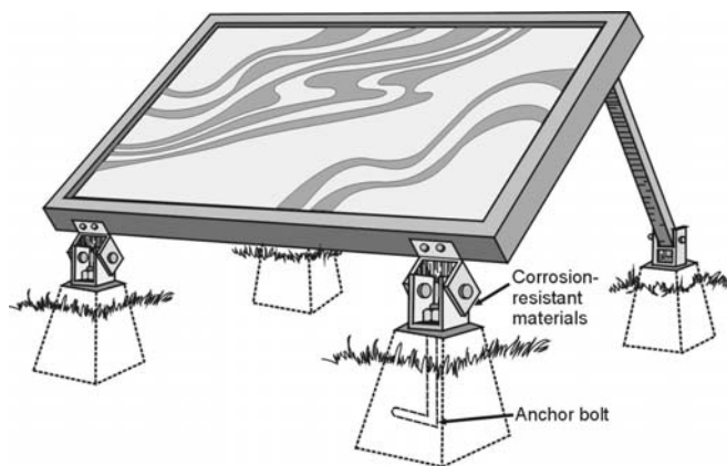
Figure 4 Ground mount
