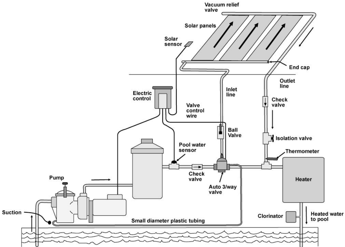
Figure 10 Plumbing schematic
