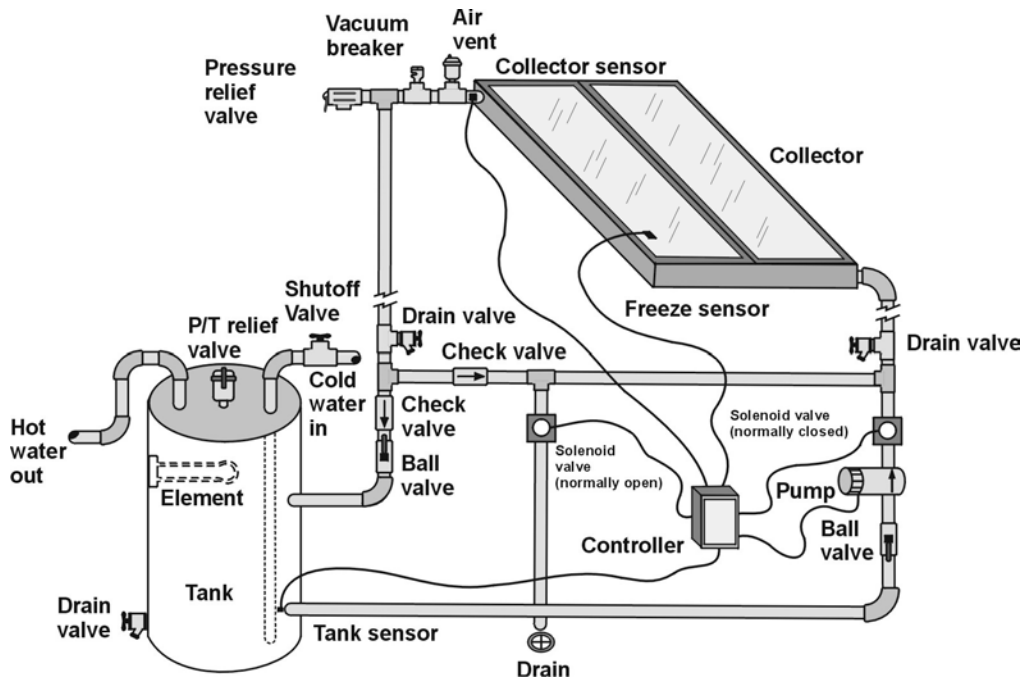
Figure 12 Drain-down system configuration
