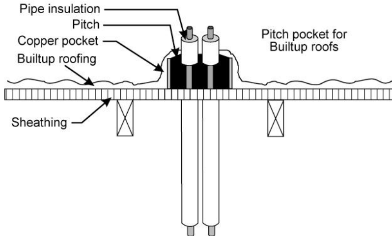
Figure 22 Penetration with pitch pocket
